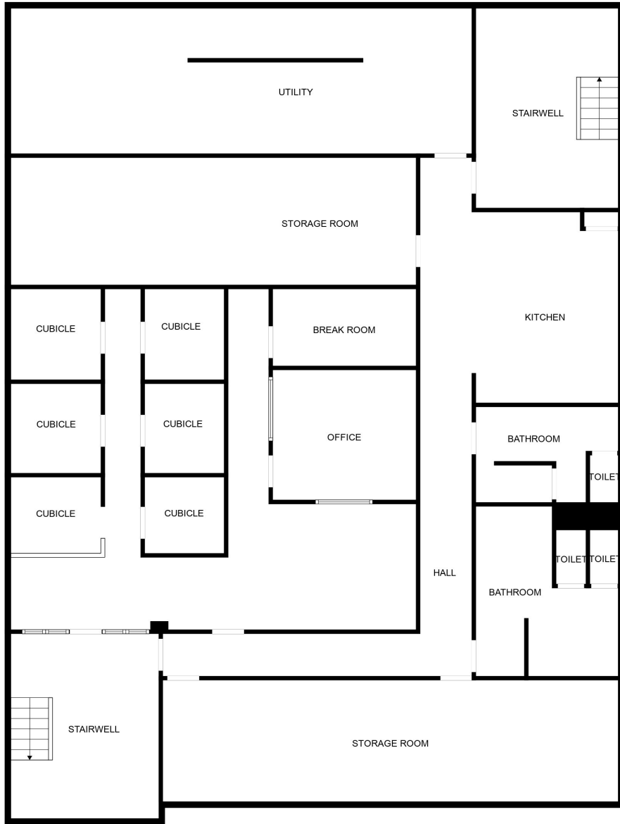
FLOOR 1
