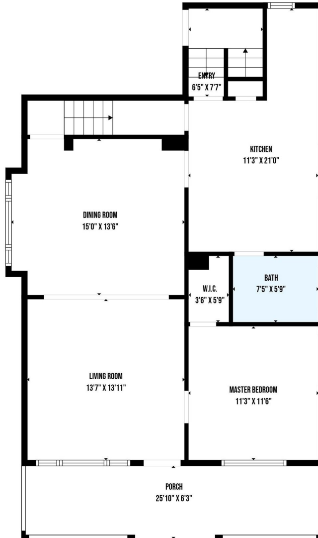
FLOOR 2
